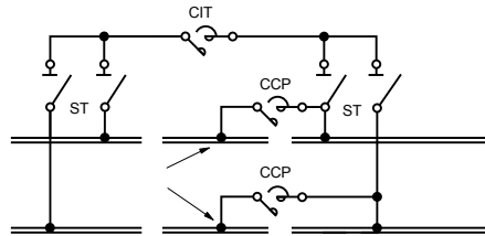
CIT, CCP: on-load switch type CMA or IF ST: disconnector type FA
